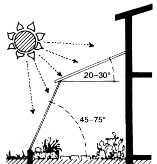
⑫ Optimal angles for glass surfaces
